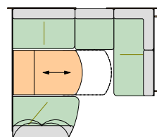
Canapé standard (894 L / 894 HS)
